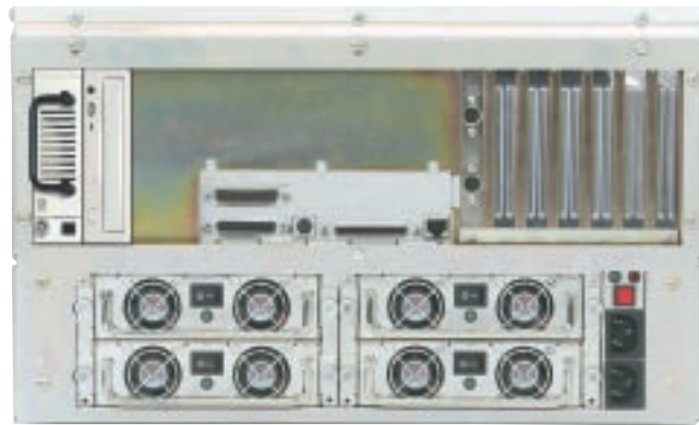
TR6 rear view with Hot swap 600W N+1 power supplies and two rear 5.25" drive bays
